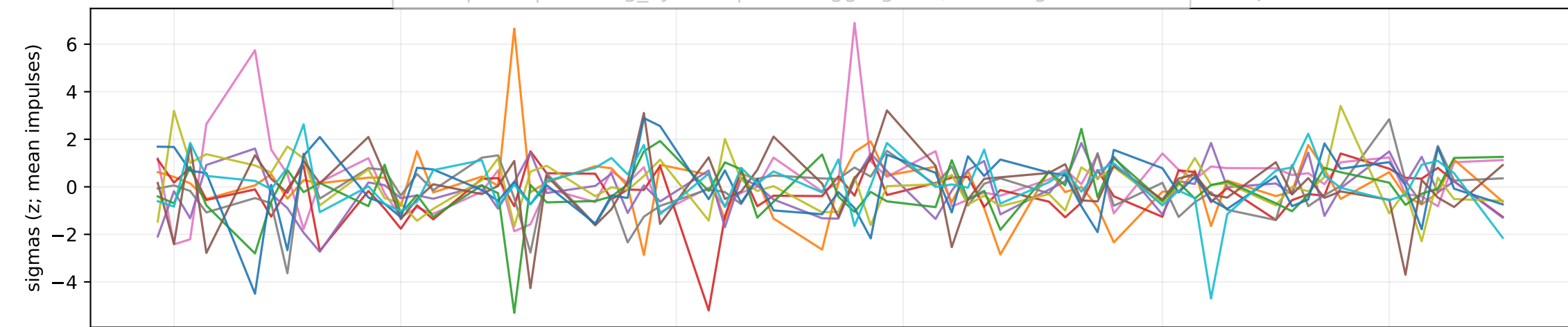
latent DEU + banking system block approximate (mean sigmas across factors)
